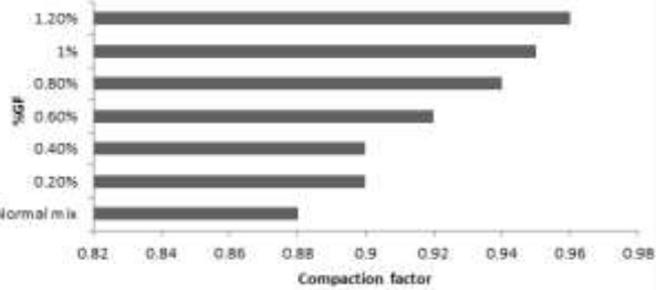
Comparison of Compaction factor with glass fibers
