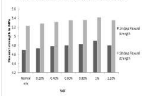
Flexural strength of concrete with glass fibers
