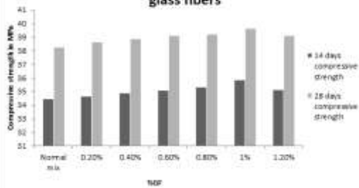
Comparison of Compressive strength with glass fibers
