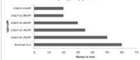
Comparison of Slump in mm with glass and polypropylene
