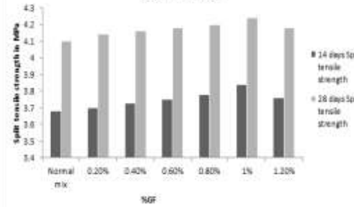
Comparison of Split Tensile strength with glass fibers
